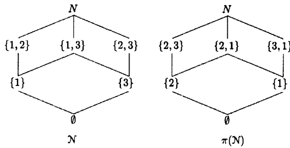
Fig. 2. Permutation of set system.
