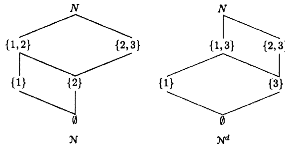
Fig. 1. Dual set system.
